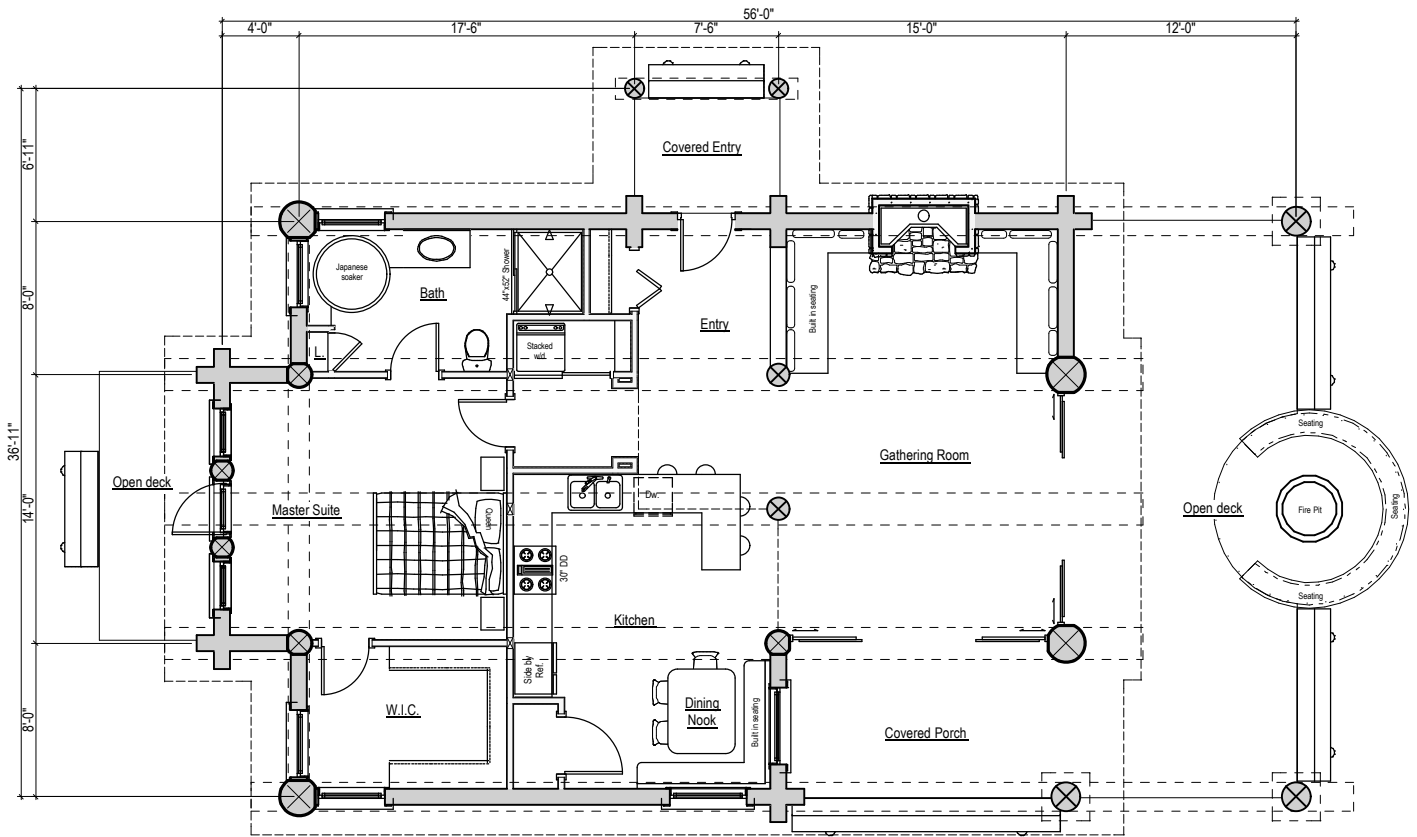
Main Level Plan
