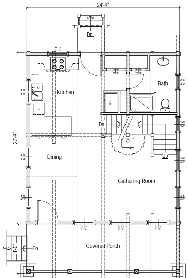
Main Level Plan
